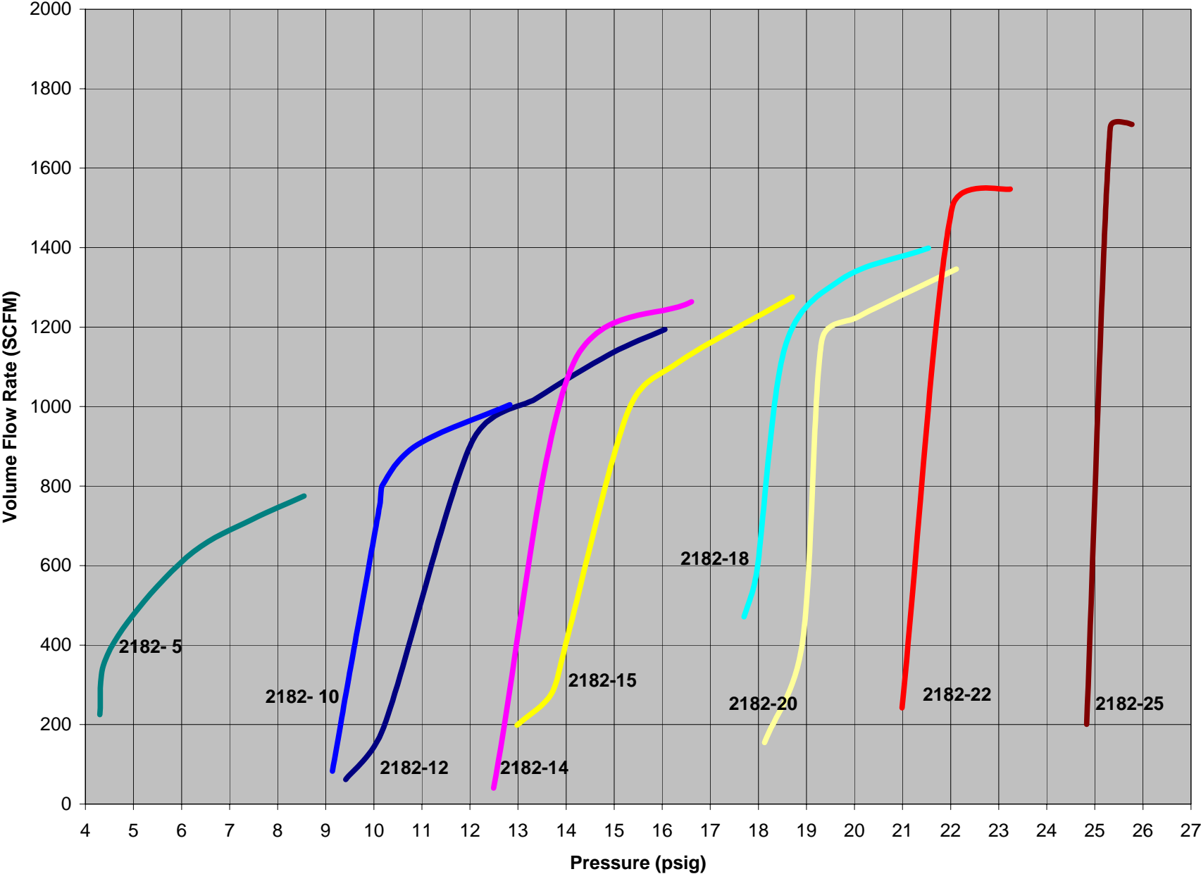
2182 Pressure Relief Valve - Flow Rate Vs Pressure
