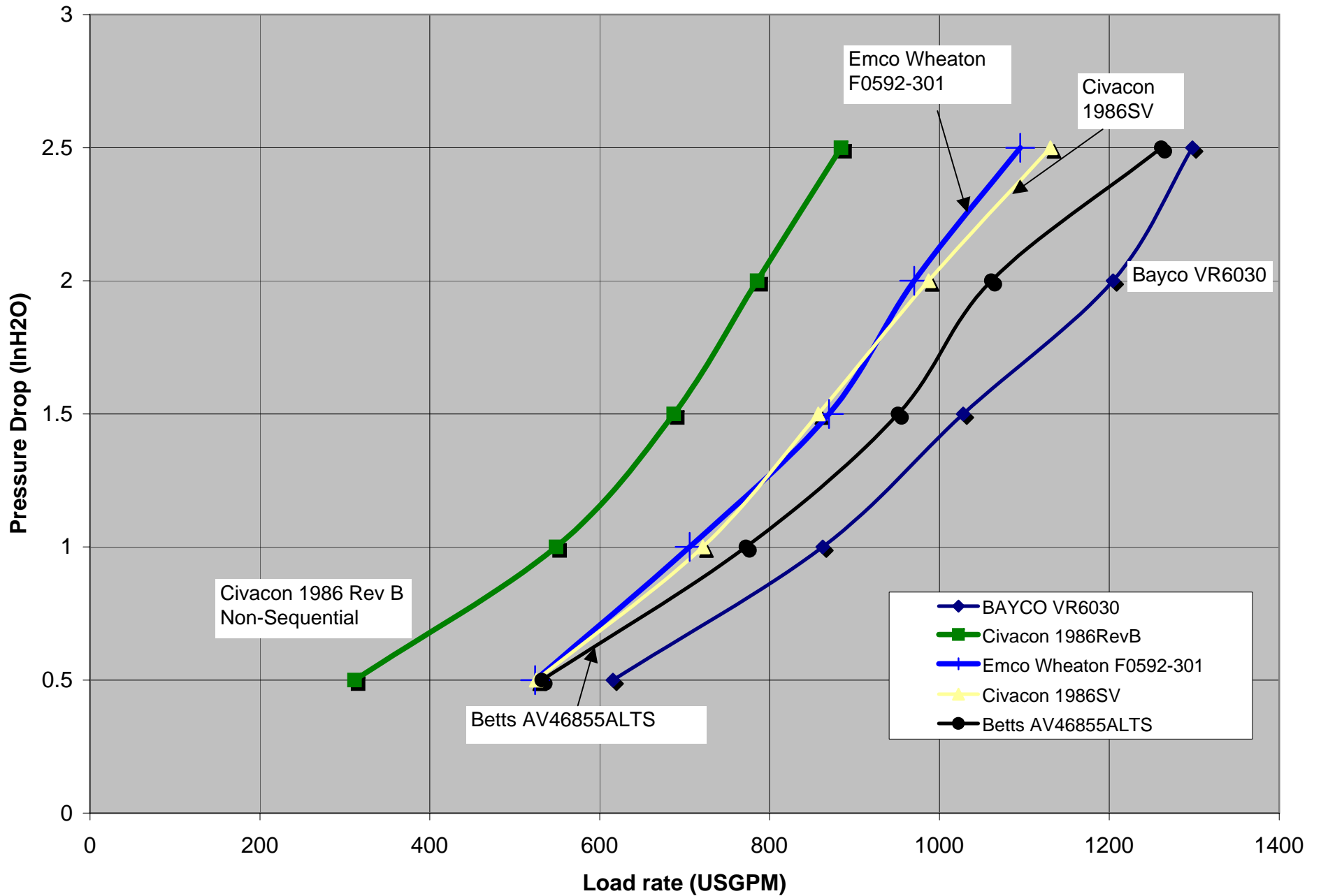
Vapour Valves (For Standard 16" Manhole Cover) - Pressure Drop Vs Flow Rate
