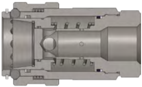
ST-Series Heavy-Duty Flush Face 'Old Style' Coupler (Female Threads)
