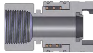
Dual-Lock P-Series Coupler (Female Threads)
