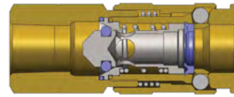
U-Series Automatic Universal Coupler (Female Threads)
