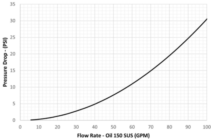
1" CNG Series - Flow Data
