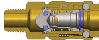
U-Series Automatic Universal Coupler (Male Threads)
