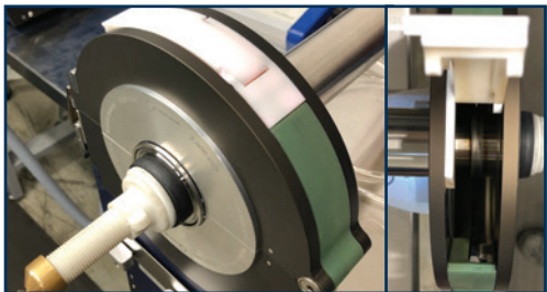
Orbital Welding
